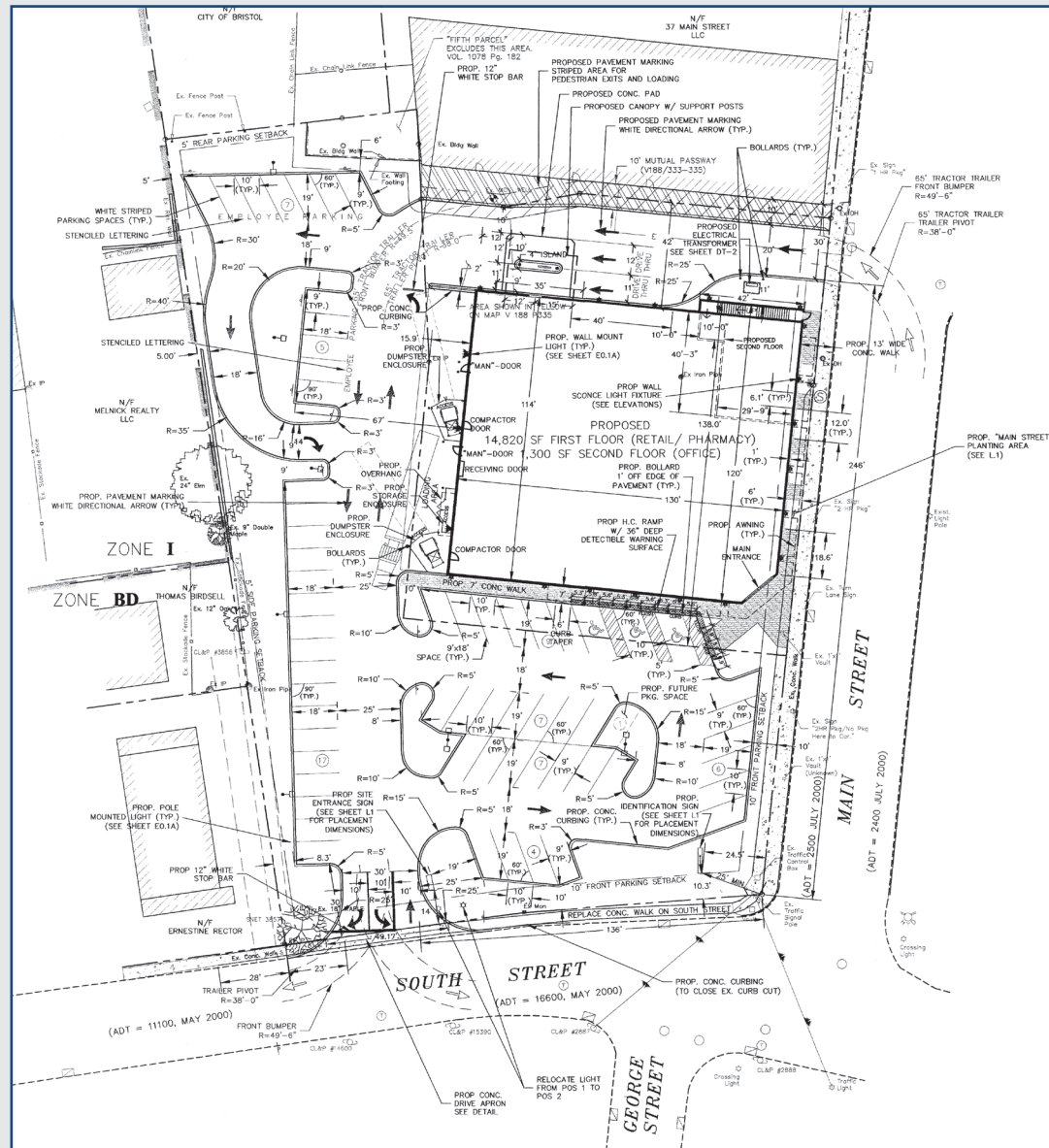
SITE PLAN
