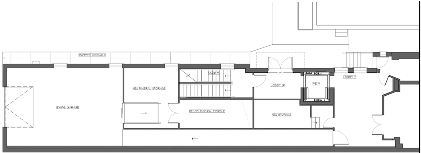
① ENLARGED PARTIAL FIRST FL. PLAN - EAST SCALE: 1/4" = 1'-0"
