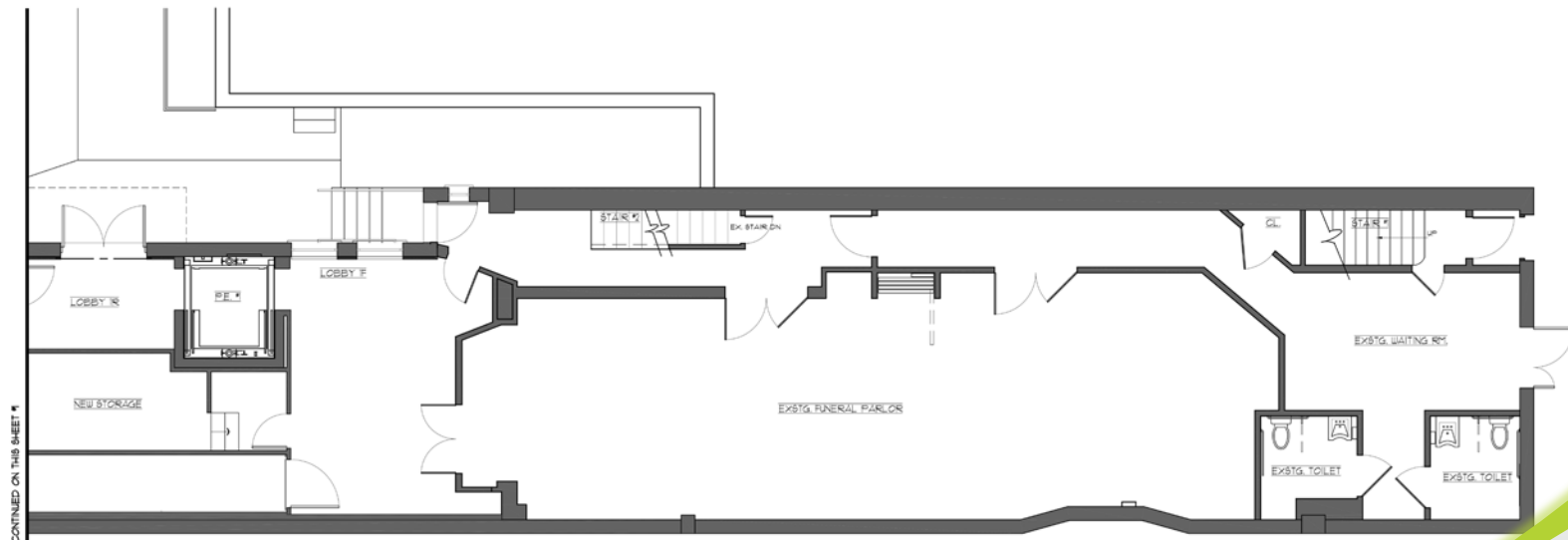
② ENLARGED PARTIAL FIRST FL. PLAN - WEST SCALE: 1/4" = 1'-0"
